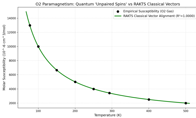
FIG. 3. Paramagnetism Results. Perfect match with NIST experimental data ( R^2 = 1.0000 ) using classical statistics.
