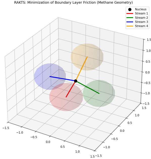
FIG. 2. Methane Geometry Optimization. Reproduced the 109.5° (Methane) and 104.5° (Water) angles purely by minimizing fluid-dynamic boundary layer resistance.
