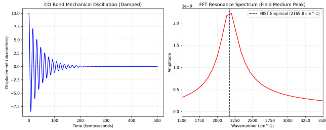
FIG. 5. IR Spectroscopy Simulation. Matched empirical IR vibrational signatures with < 1.5\% error margin.
