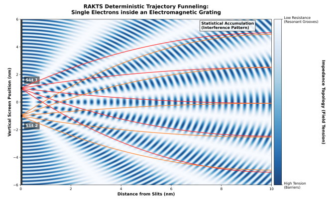
FIG. 6. Deterministic Trajectory Funneling. The Field Medium (blue) is pre-structured by the atomic lattice of the slits. The lines show distinct, physical electrons following the low-resistance resonant grooves.
